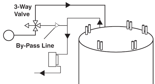
(Optional) Hot Gas By-Pass Valve Example
