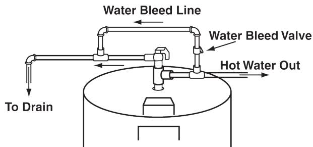
(Optional) Water Bleed Valve Example
