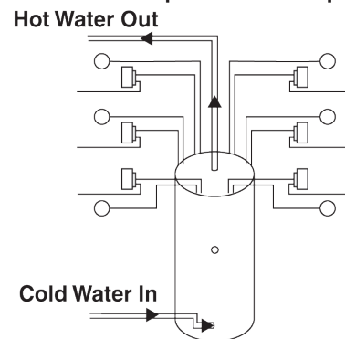
6 Compressor Example
